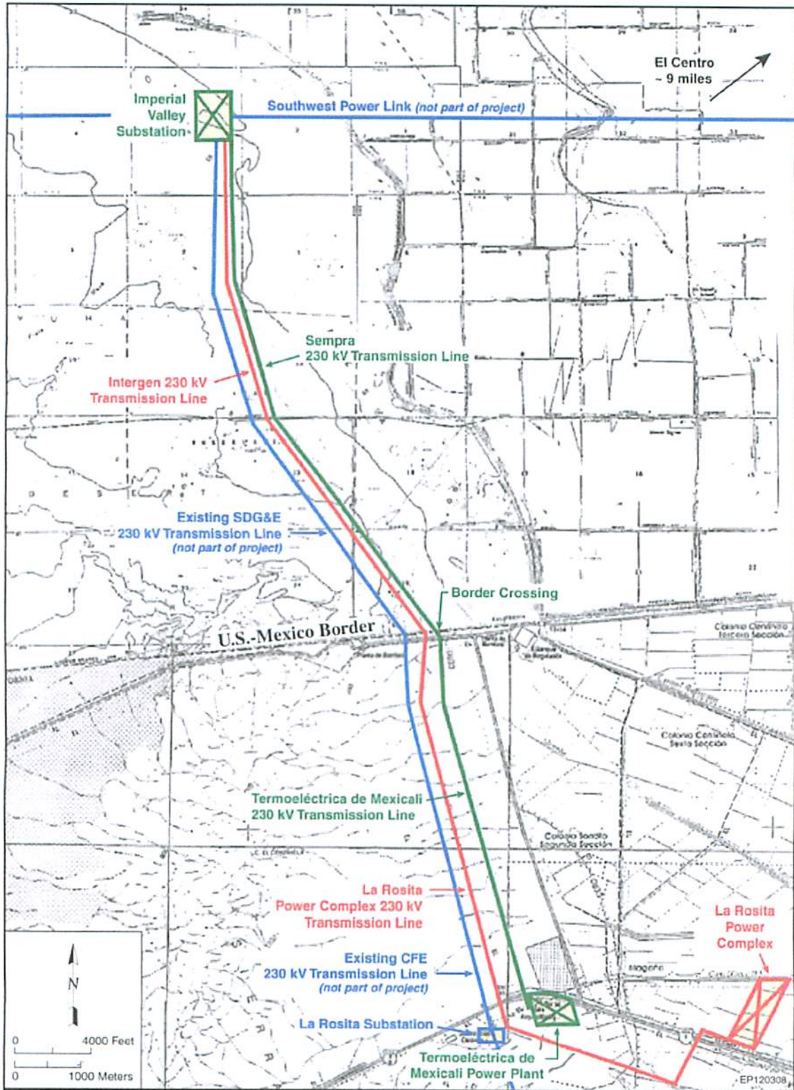
FIGURE S-1 General Area Map Showing the Proposed Transmission Lines
